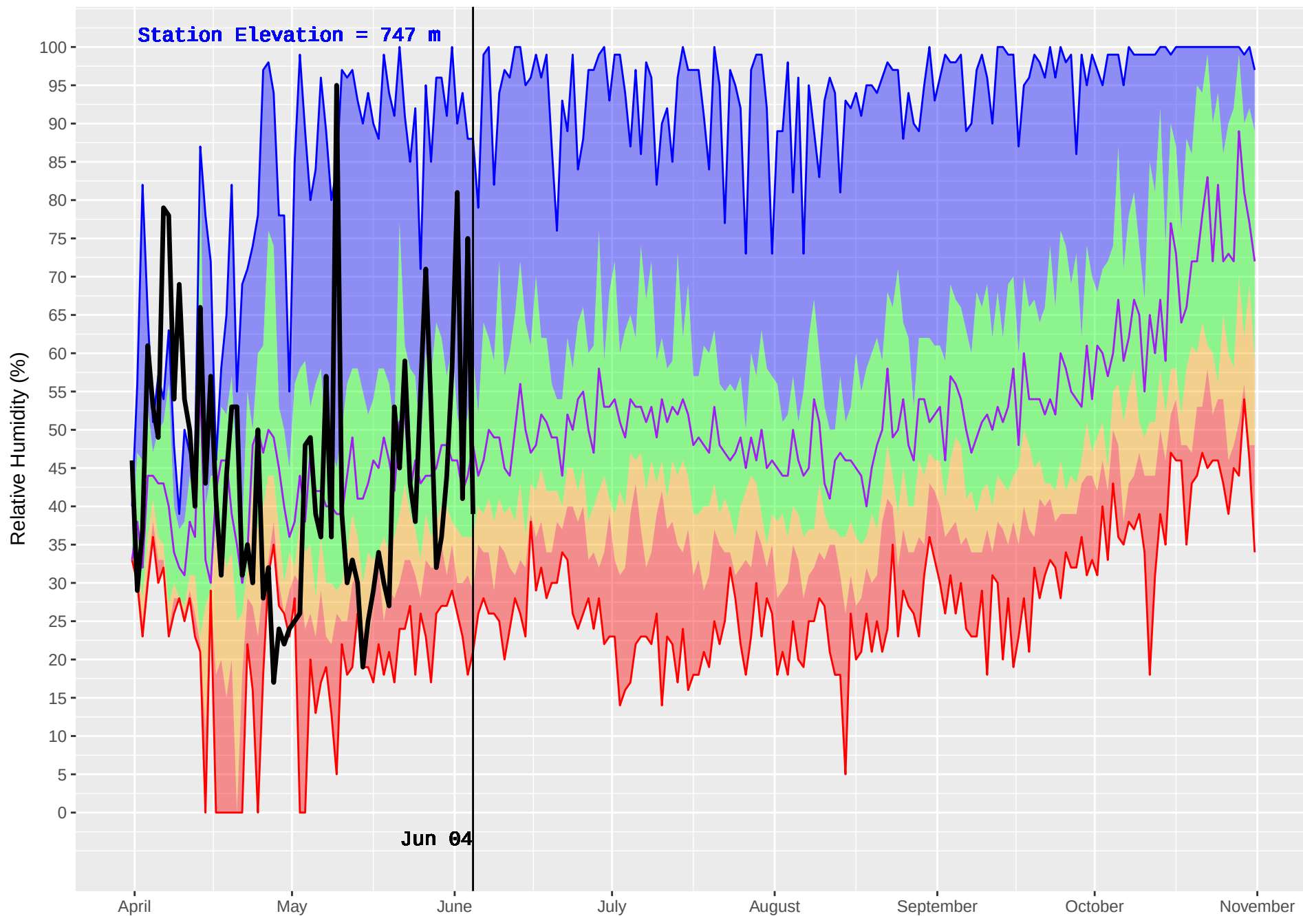
PEDEN (178) : Historical (1984–2016) and Current (2018) Noon Relative Humidity
