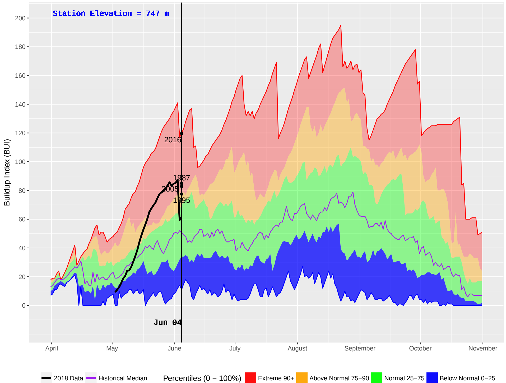
PEDEN (178) : Historical (1984–2016) and Current (2018) Noon Buildup Index (BUI)
