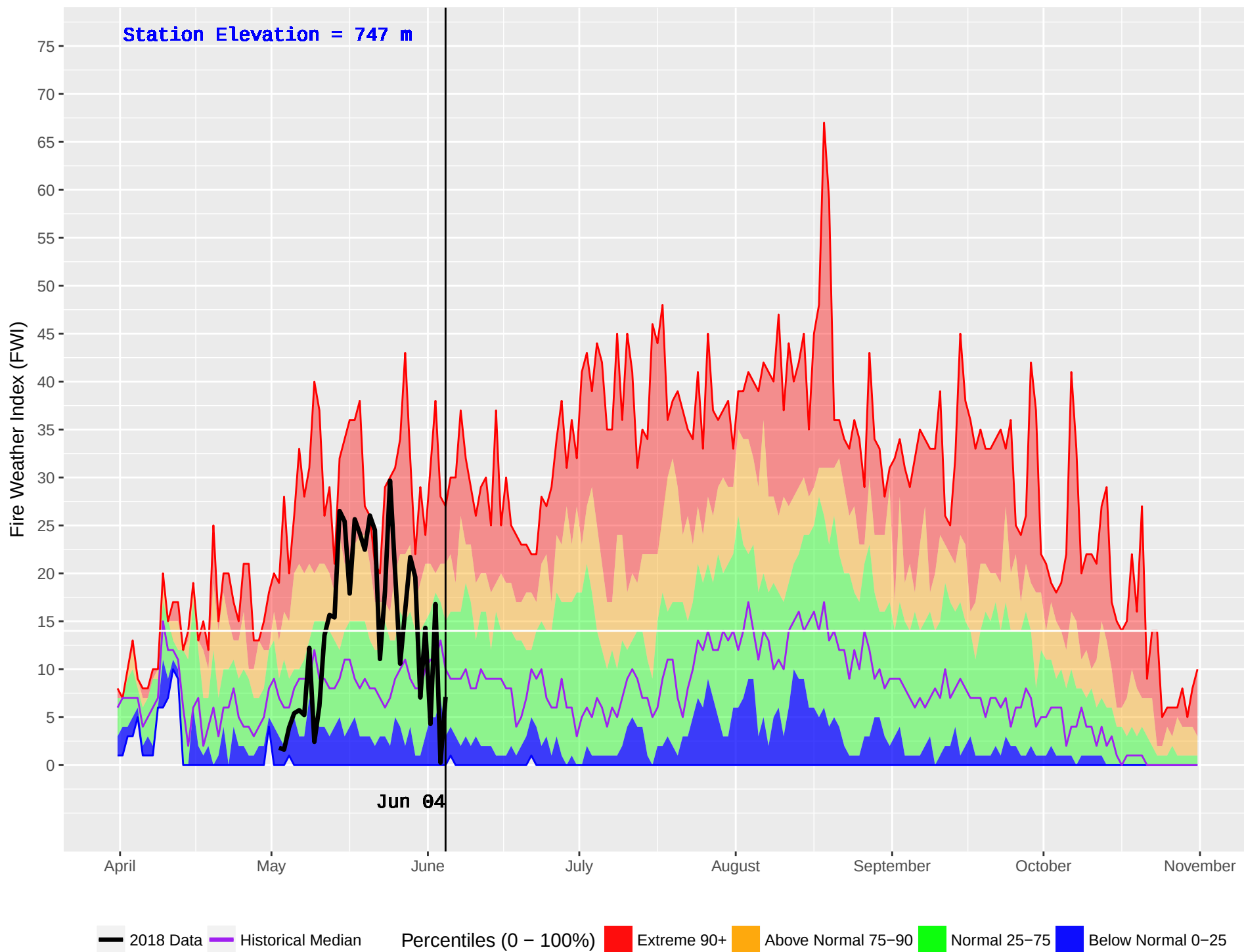
PEDEN (178) : Historical (1984–2016) and Current (2018) Noon Fire Weather Index (FWI)
