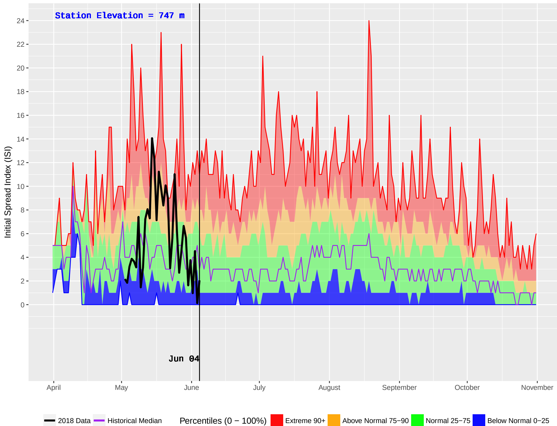
PEDEN (178) : Historical (1984–2016) and Current (2018) Noon Initial Spread Index (ISI)
