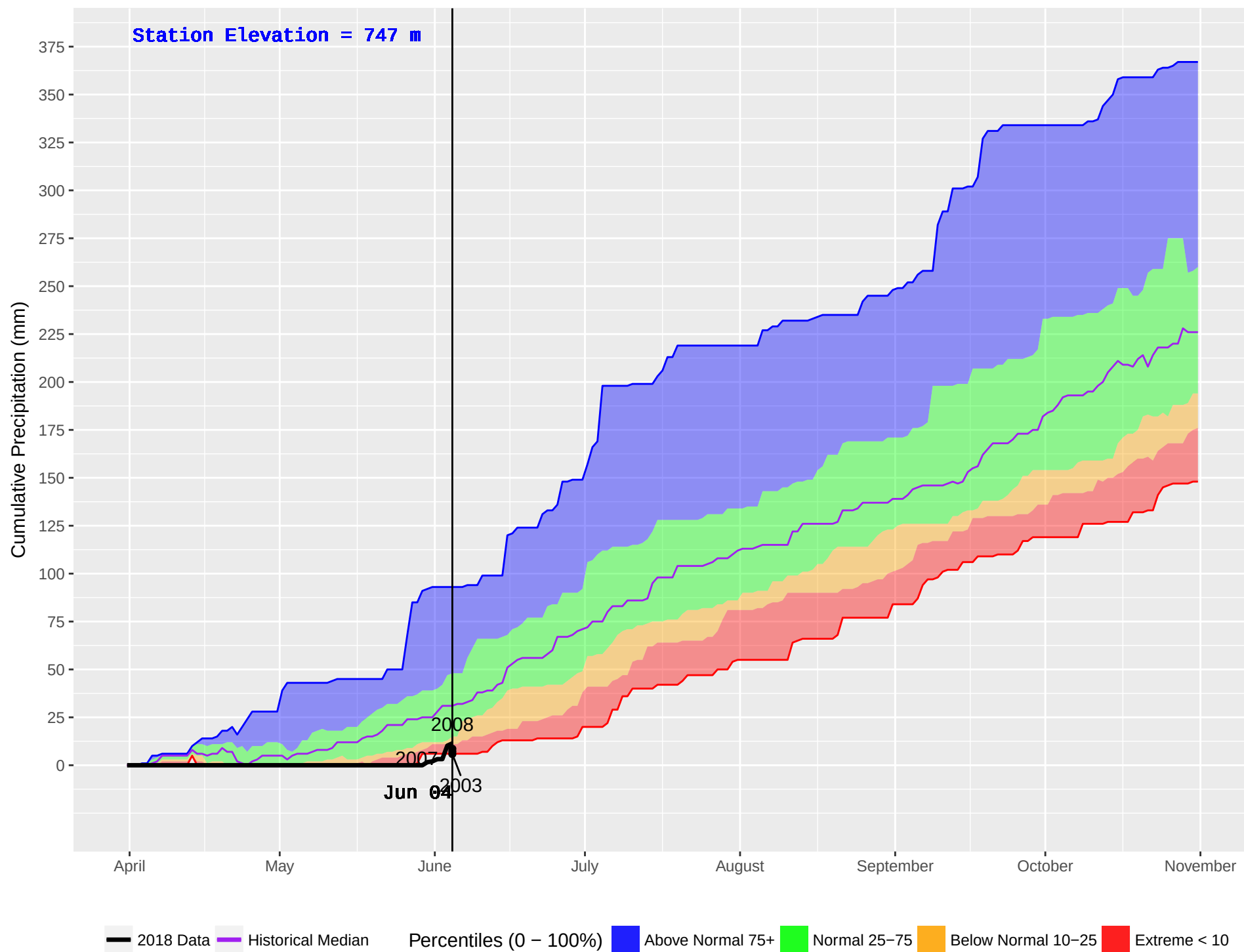
PEDEN (178) : Historical (1984–2016) and Current (2018) Noon Cumulative Precipitation
