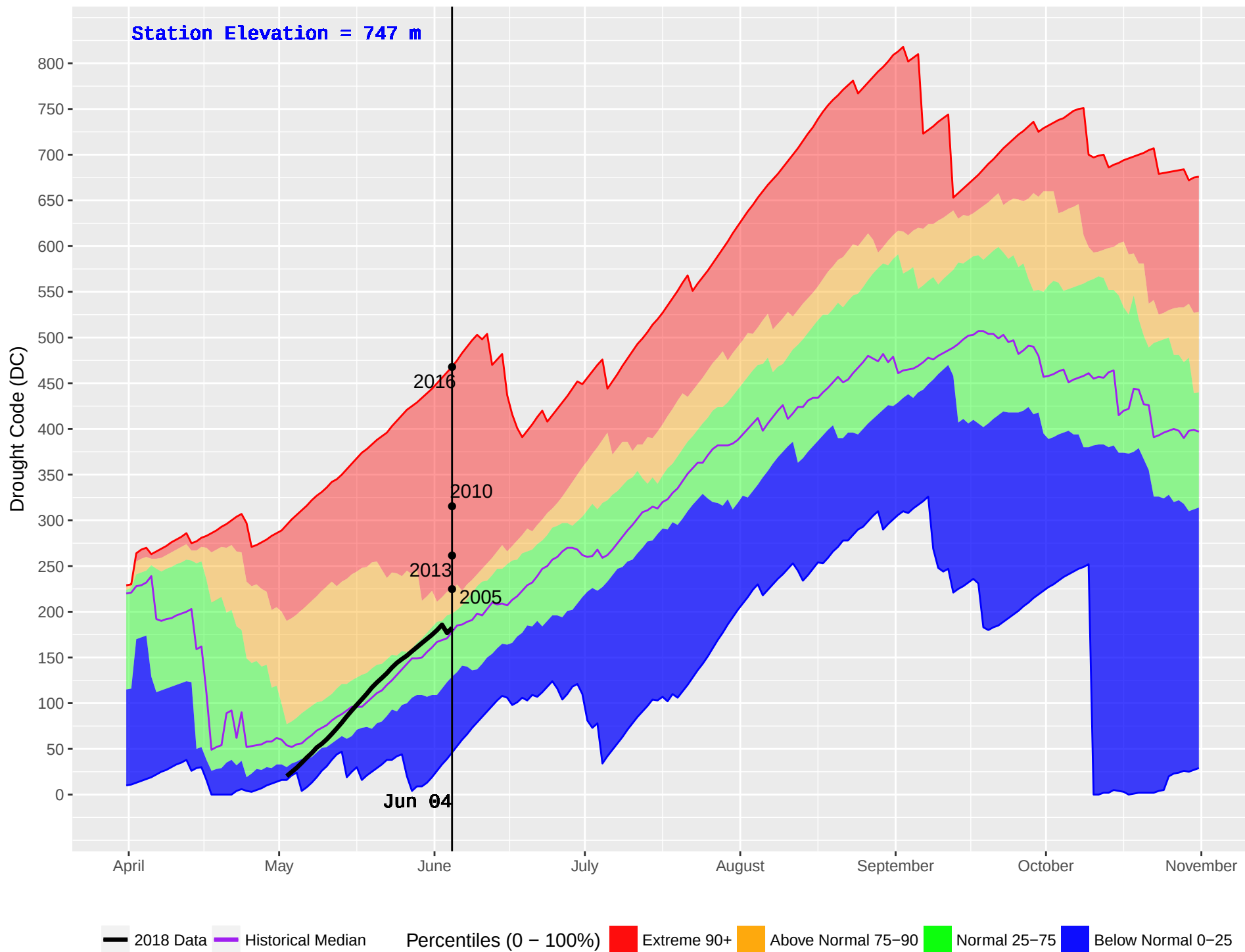
PEDEN (178) : Historical (1984–2016) and Current (2018) Noon Drought Code (DC)
