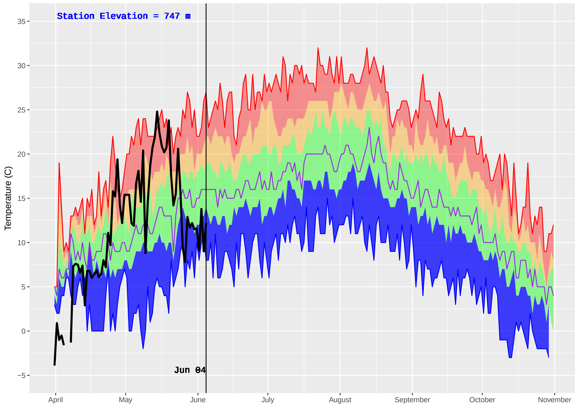
PEDEN (178) : Historical (1984–2016) and Current (2018) Noon Temperature
