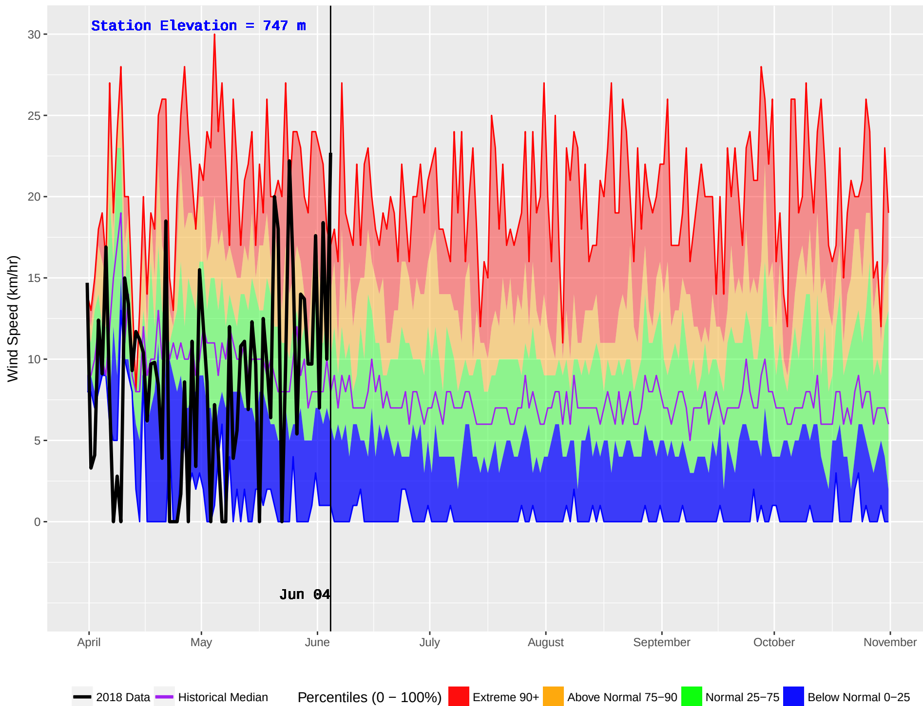
PEDEN (178) : Historical (1984–2016) and Current (2018) Noon Wind Speed
