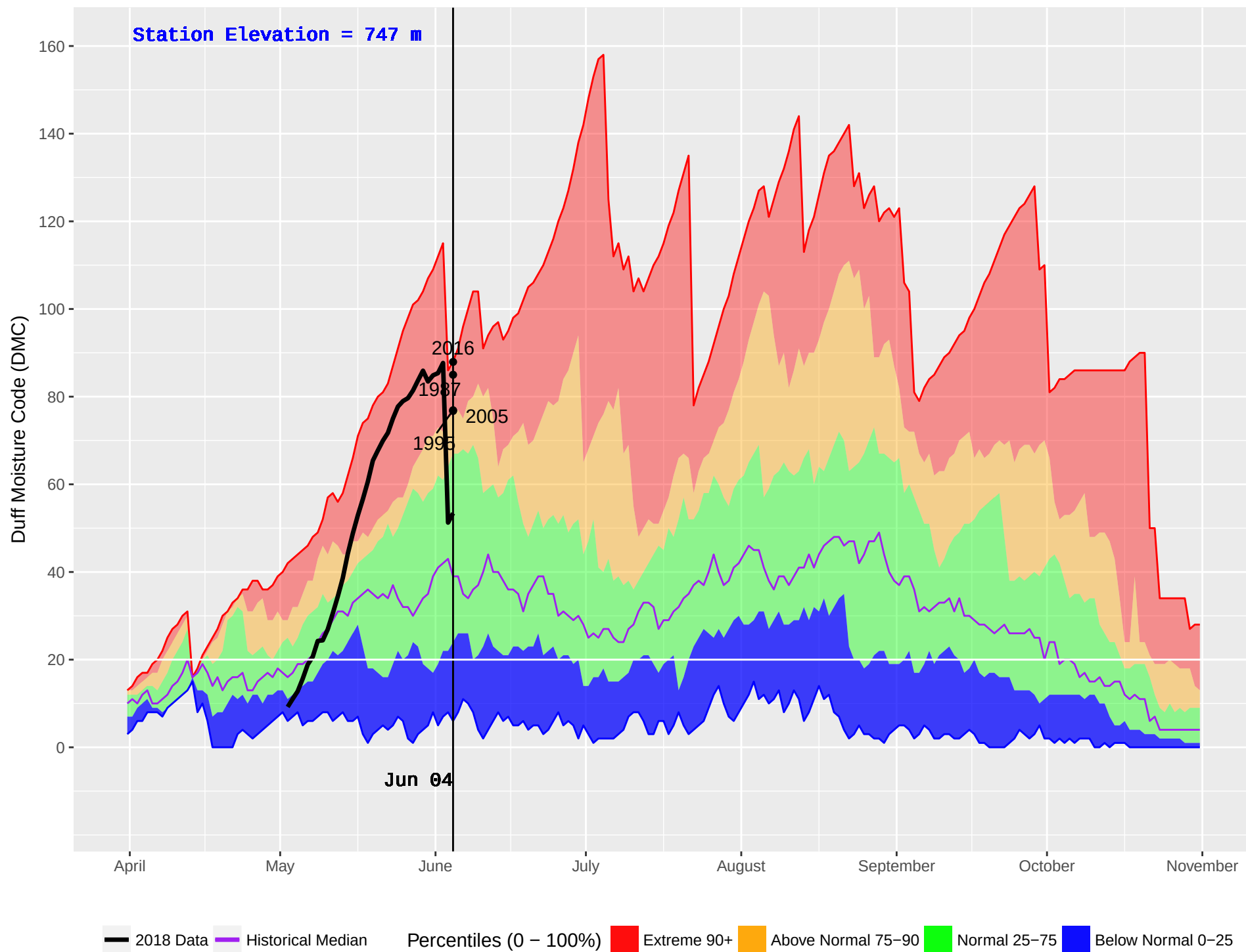
PEDEN (178) : Historical (1984–2016) and Current (2018) Noon Duff Moisture Code (DMC)
